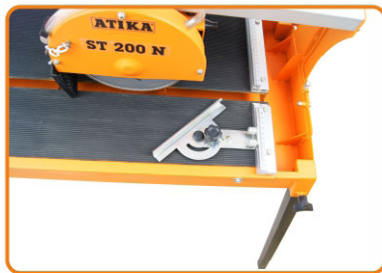
angle fence for mitre cuts
